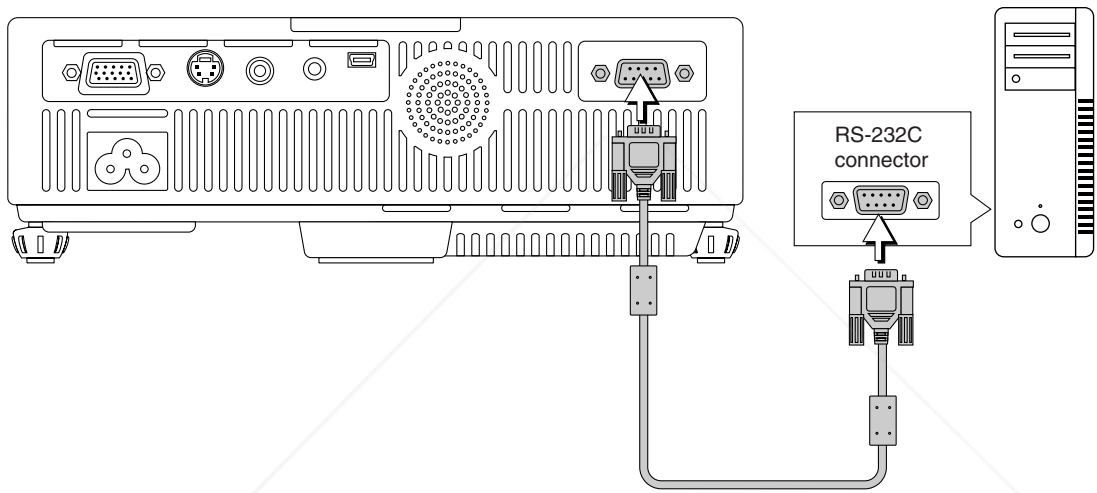
Serial cable (D-Sub 9-pin, straight) (commercially available)
