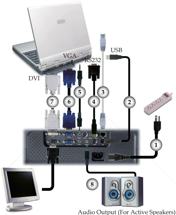
Audio Output (For Active Speakers)
