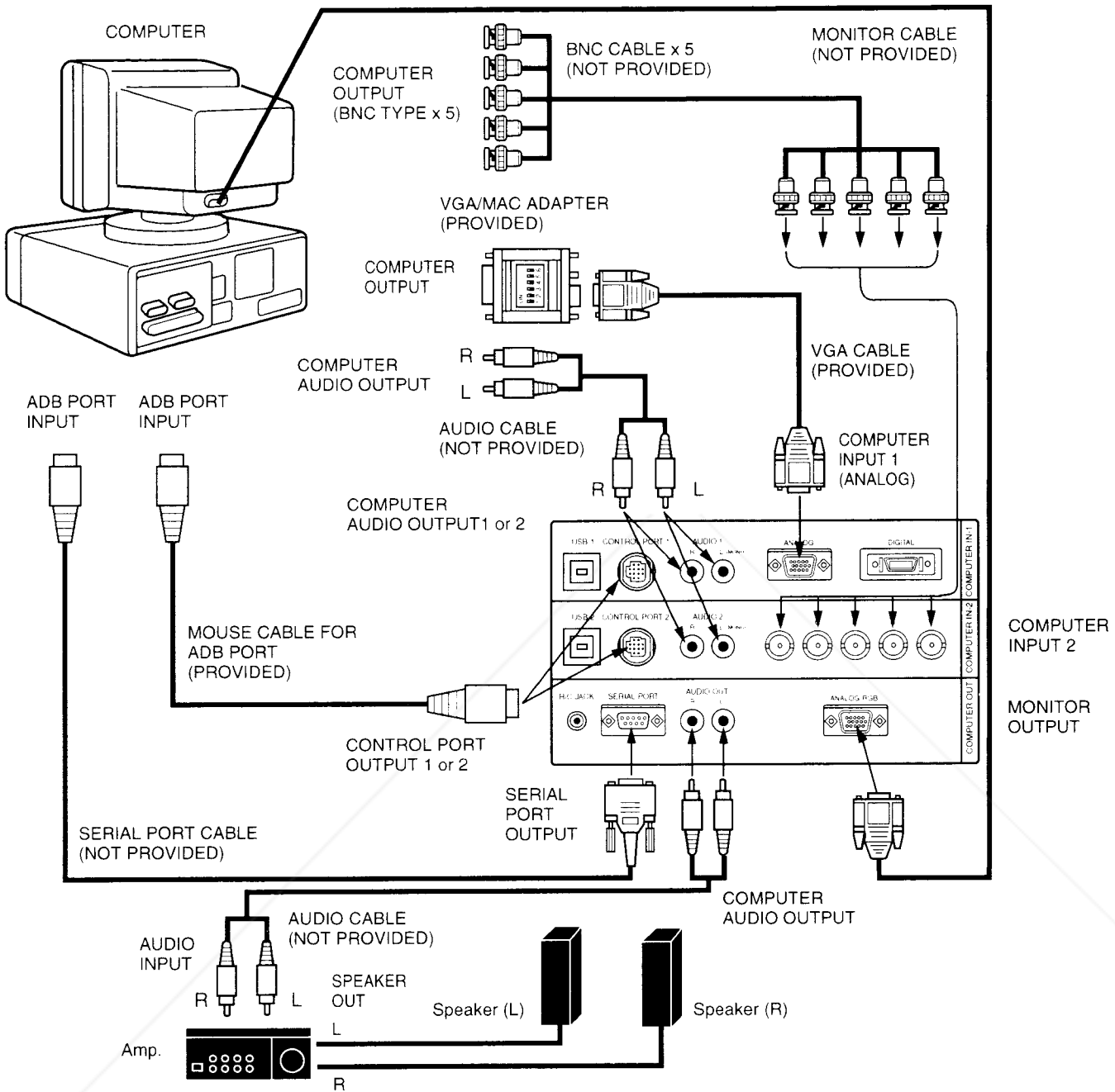
VGA/MAC ADAPTER
