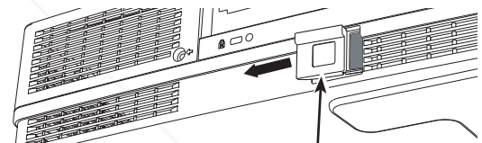
Air filter (back) Pull horizontally and then remove it leftward.
