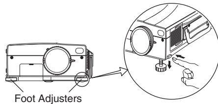
Foot Adjusters
