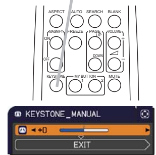
KEYSTONE button
