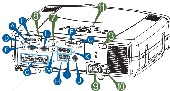
Projector (Rear/Left)
