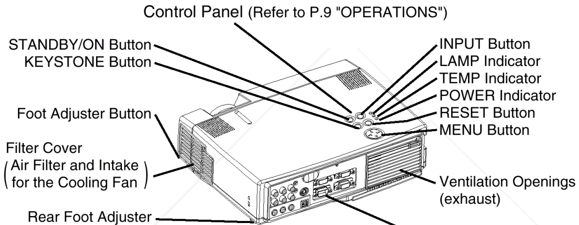
REAR/RIGHT VIEW OF THE PROJECTOR
