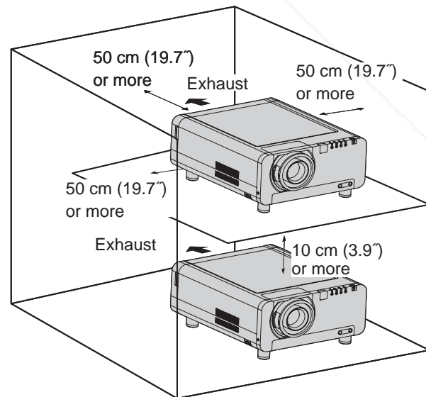
(Figure 2 : Dimensions applying when two units are used)
