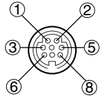
DIN 8-PIN connector seen from outside
