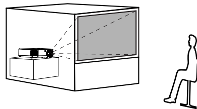
INSTALLATION: REAR/DESK
