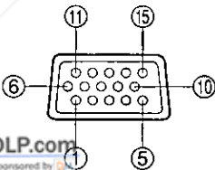
External view
