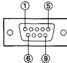
D-Sub 9-pin (male) external appearance
