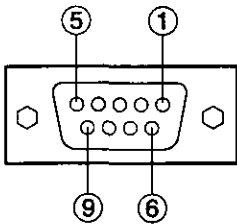
D-Sub 9-pin (female) external appearance
