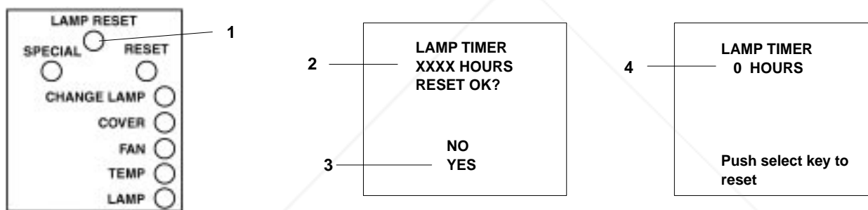
Figure 6-1. Projector Control Panel
