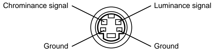
S VIDEO input (Mini DIN4 pin)
