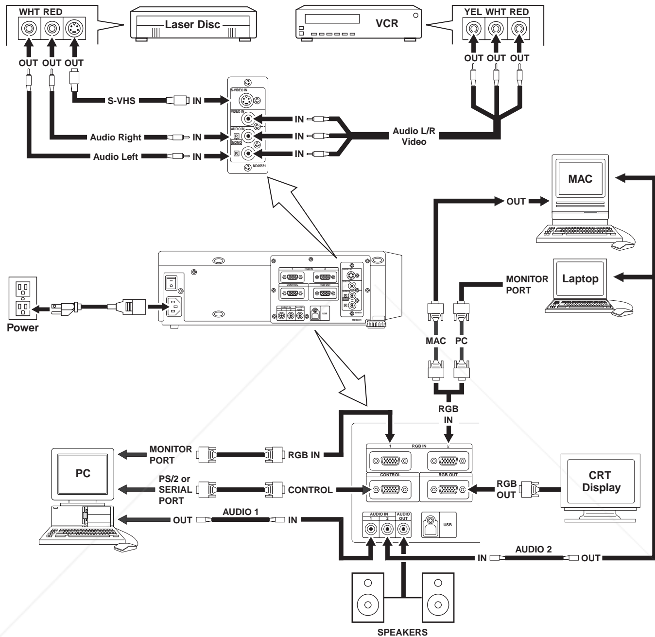
Figure 2.3 Cable Connections
