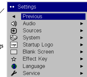
Settings menu
