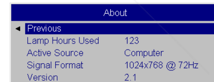
About menu
