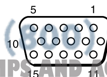
D-sub 15 pin terminal (Female)
