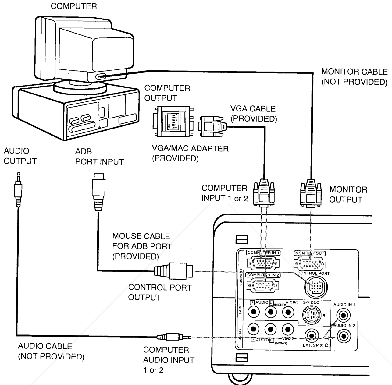
VGA/MAC ADAPTER
