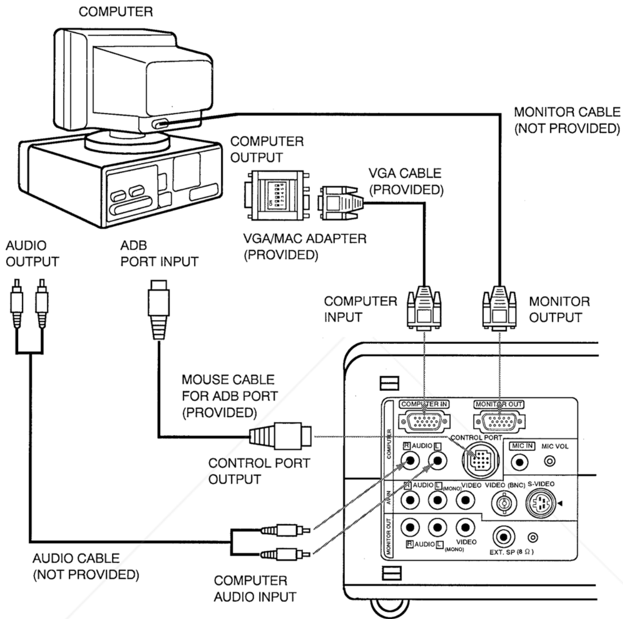
VGA/MAC ADAPTER
