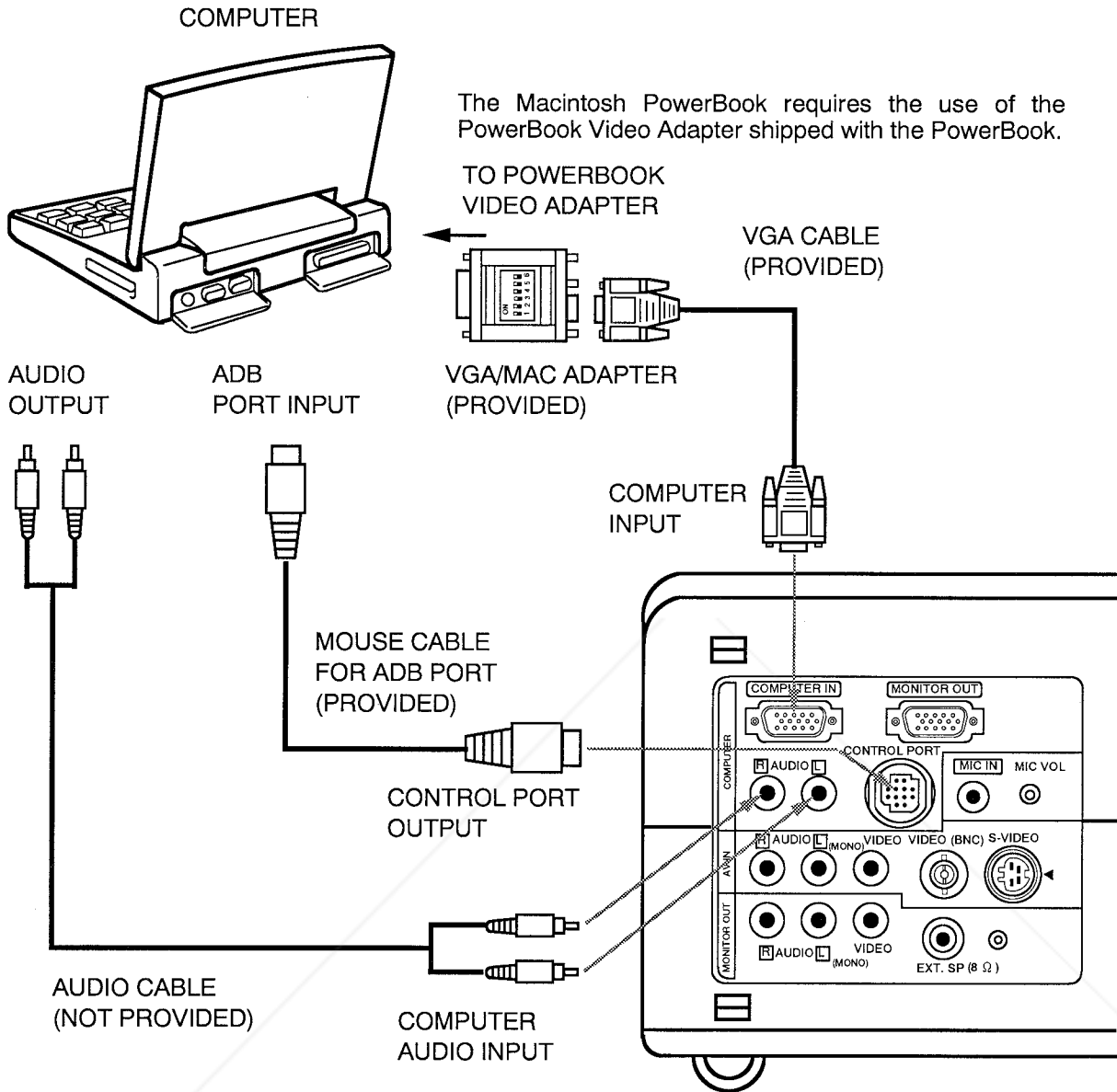
VGA/MAC ADAPTER
