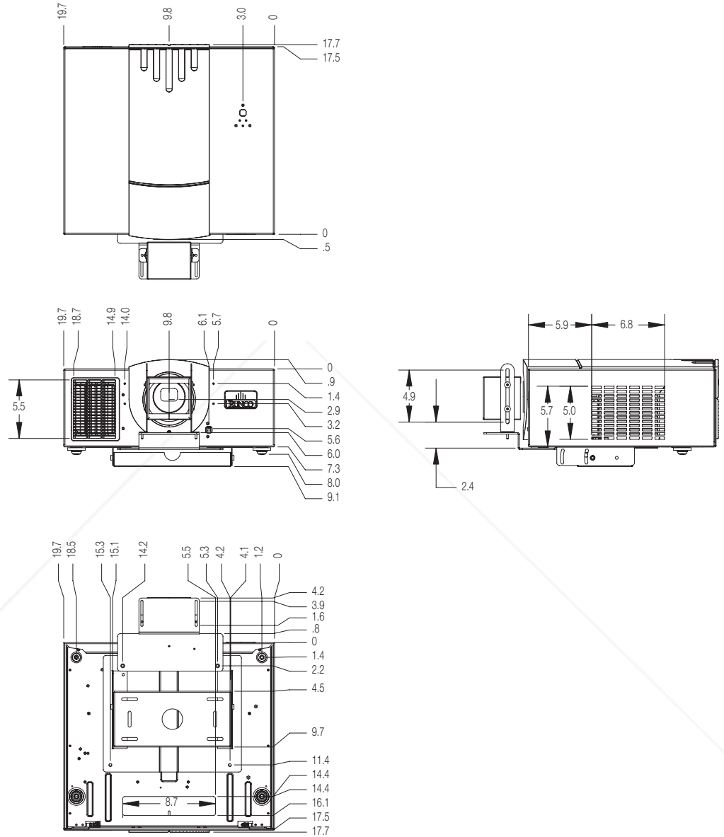
Figure 7-1. Overall Dimensions – VX-3000i/CineWide and VX-3000d/CineWide (Prismatic Lens)
