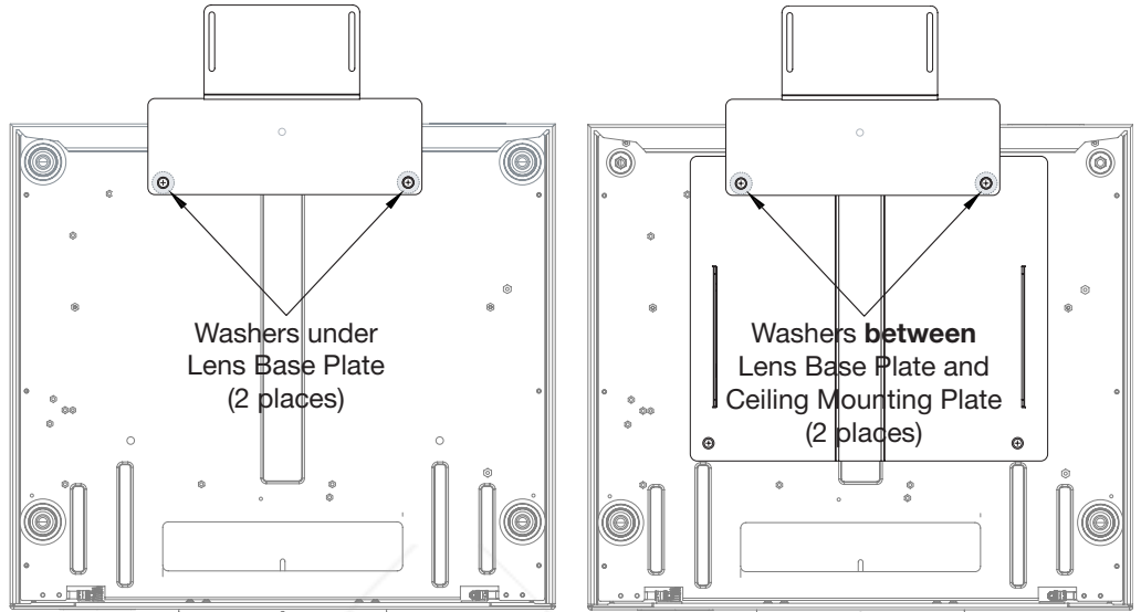
VX-3000i/CineWide or VX-3000d/CineWide with Prismatic Lens Base Plate and Ceiling Mounting Plate
