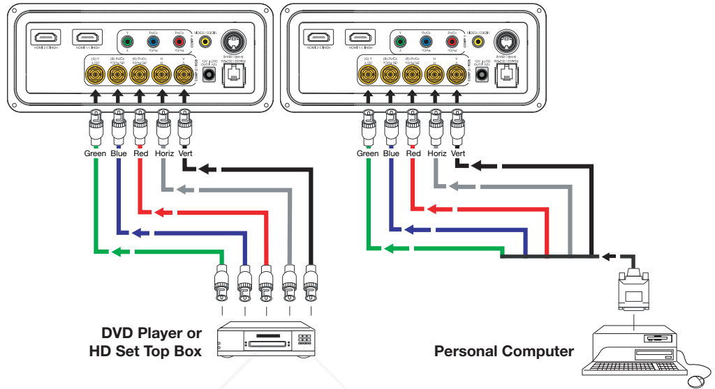
Figure 3-14. RGB Connections
