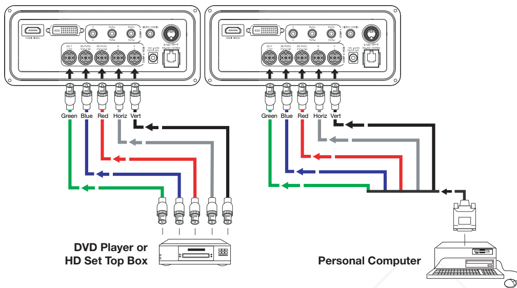
Figure 3-8. RGB Connections
