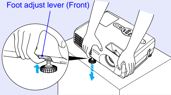
Foot adjust lever (Front)
